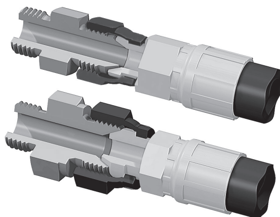
Fig. G1 – JIS T4 and P4 Interfaces
